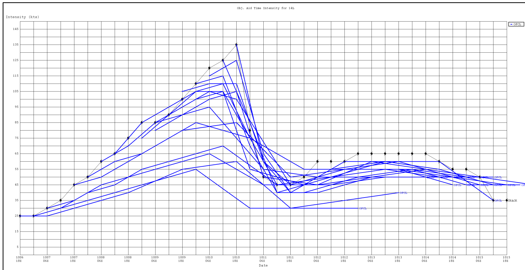
Figure 12. Selected NHC official intensity forecasts (kt, blue lines) for Hurricane Michael. The best track intensity (kt) is given by the black line with the symbols at 6 h interval.
